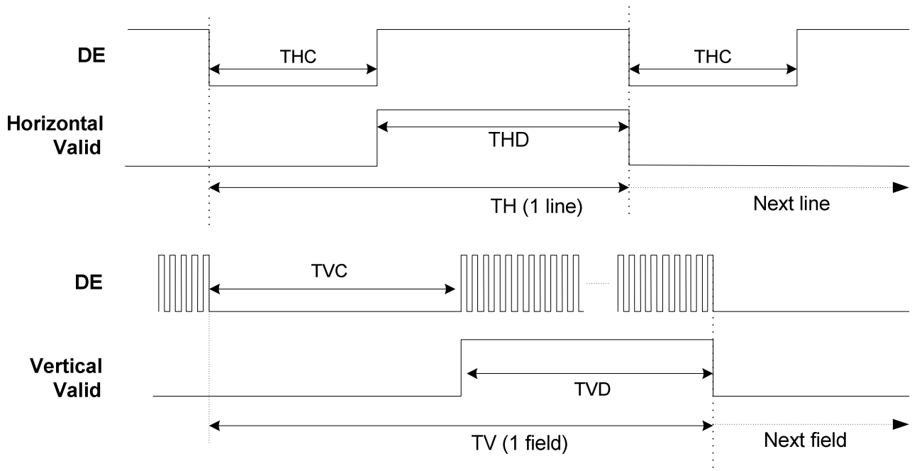
Fig.3-2 DE Mode Input Timing
