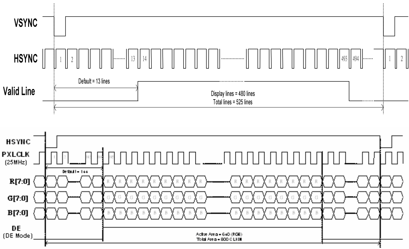
Fig. 3-4 24 bit RGB mode for 640 x(RGB)x 480
